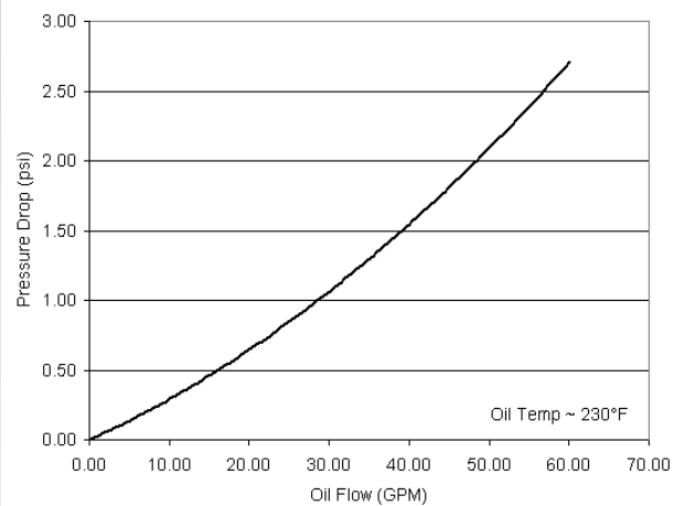
TDI-18316 Oil Side Pressure Drop
