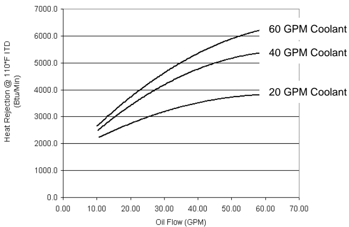
TDI-18316 Oil Heat Rejection
